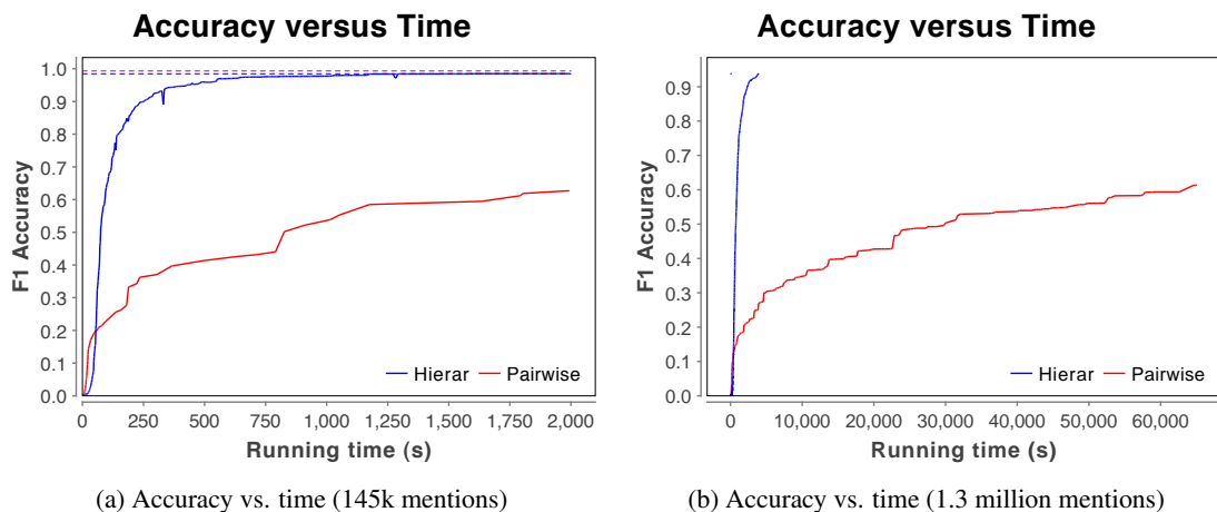
Figure 5: Runtime performance on two datasets
